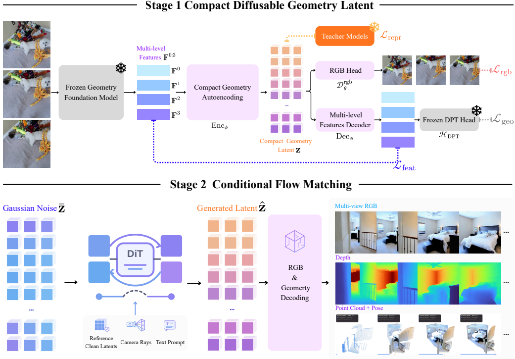
Figure 2: Overview of Geometry-Native Autoencoder (GAE). Stage 1 (codec training) compresses frozen multi-level geometry foundation features into a compact, diffusable geometry latent; the feature decoder rebuilds the full hierarchy for frozen geometry readout, while a separate learned head decodes RGB. Stage 2 (flow training) performs conditional flow matching only over generated-view latents, while clean reference latents, camera rays, and text act as controls.
