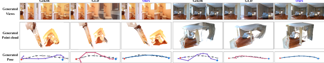
Figure 6: Multi-frame RGB, geometry, and camera-pose comparison across RealEstate10K scenes. Gen3R, GLD, and Ours receive the same reference image and prescribed camera trajectory. For each scene, early, middle, and final generated views are paired with the generated point cloud and recovered pose. The multi-scene comparison exposes cross-frame structure, depth-layer distortions, and trajectory drift that are less apparent in a single final view.
